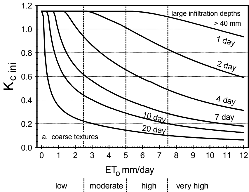
FIGURE 30 Average K_{c\ ini} as related to the level of ET_0 and the interval between irrigations greater than or equal to 40 mm per wetting event, during the initial growth stage for a) coarse textured soils; b) medium and fine textured soils
