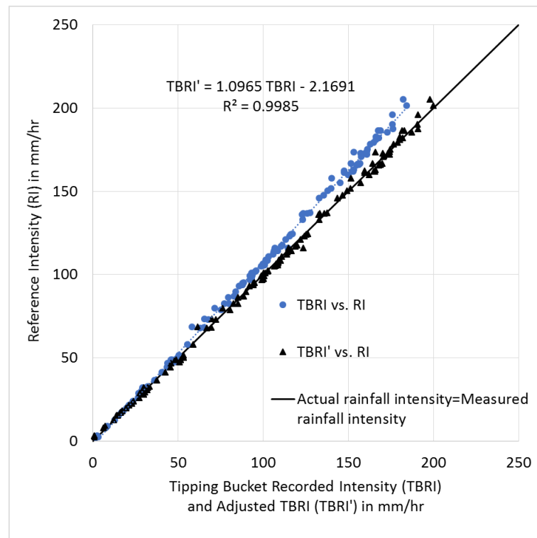
Figure 3 Tipping Bucket Rain Gauge Calibration Curve
