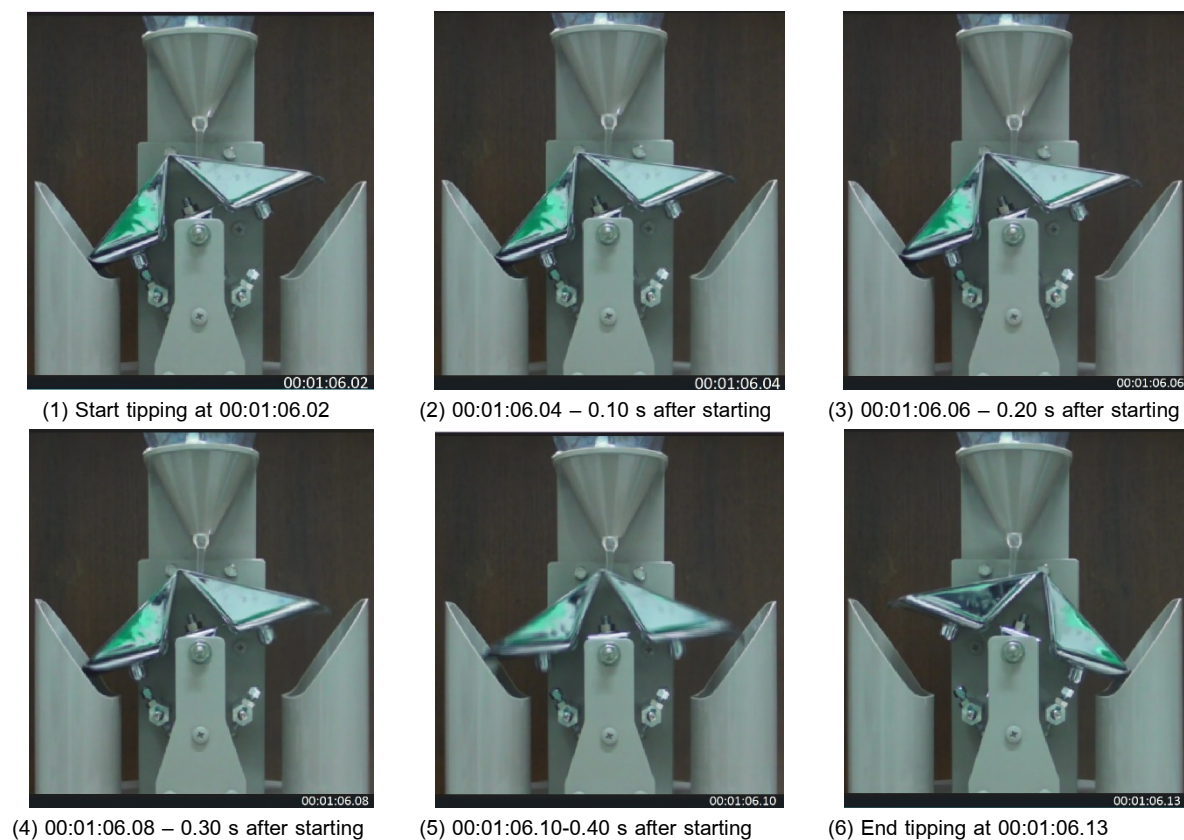
Figure 6 Photos from Video Recorder Showing Time in Decimal of Second During Bucket Tipping from Start to End for 114 mm/hr Reference Intensity
