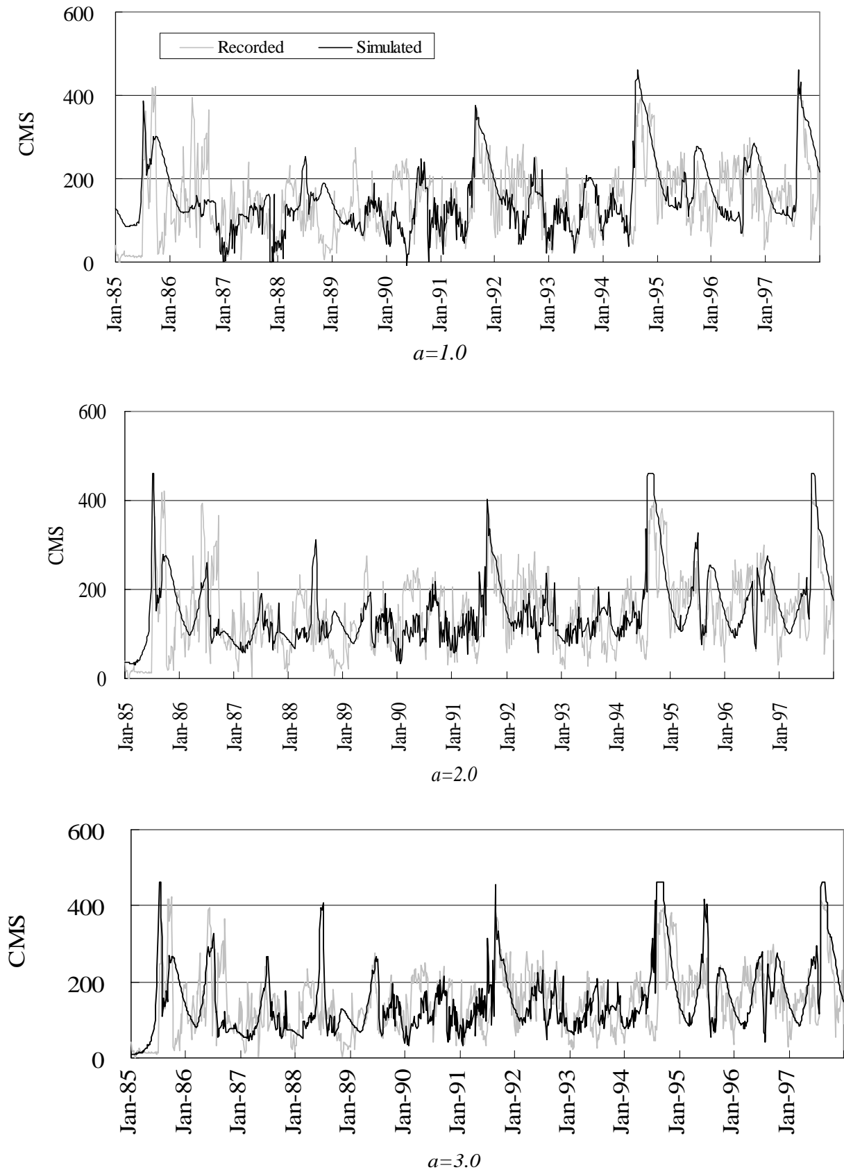
Fig. 13. Simulated Release from SRN Dam at Different a Values.
