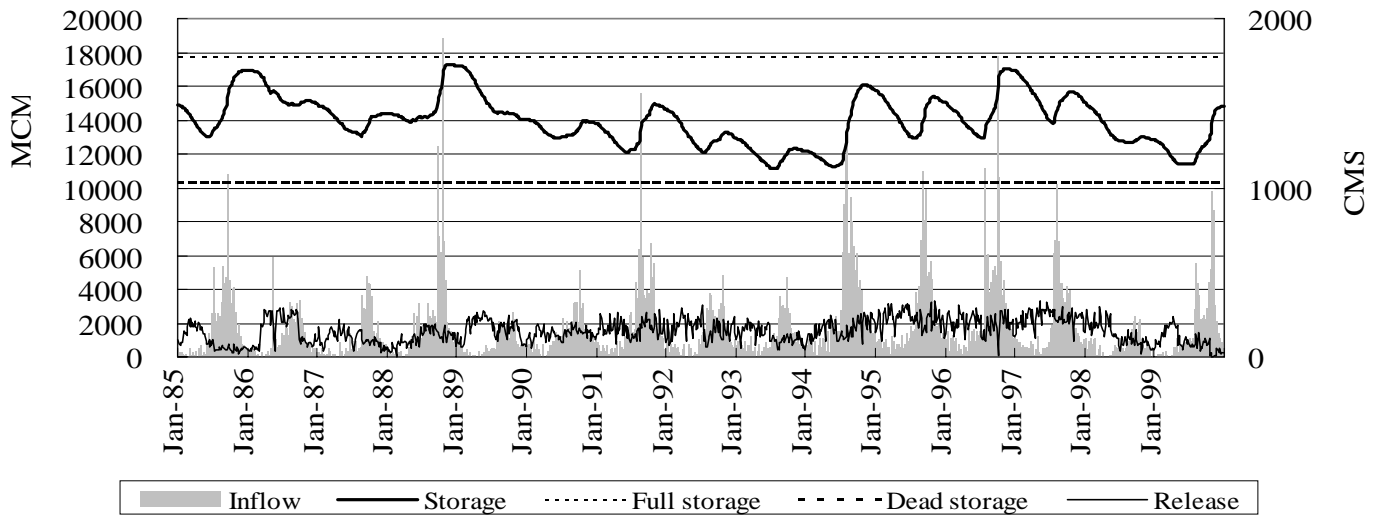
Fig. 1. Reservoir Operation Record (SRN)
