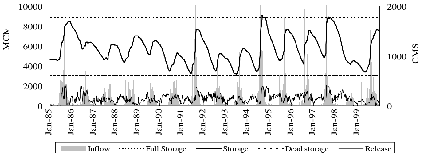
Fig. 2. Reservoir Operation Record (KHL)
