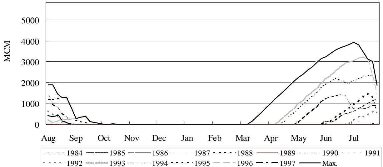
Fig. 8. Seasonal Vacancy Requirement (KHL)
