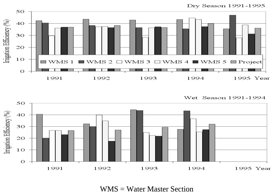
Figure 4 Irrigation efficiency of Song Phi Nong Irrigation Project and 5 water master sections during 1991-1995.
