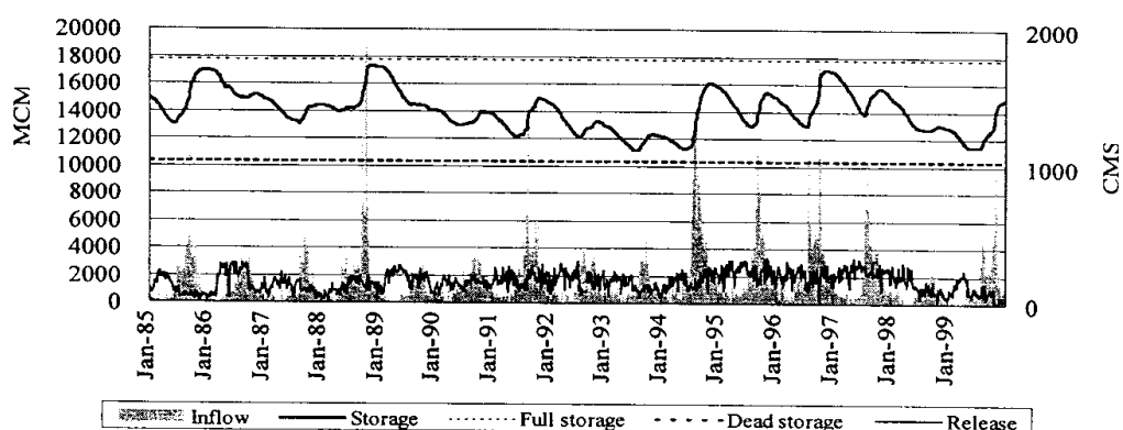
Fig. 1. Reservoir Operation Record (SRN)
