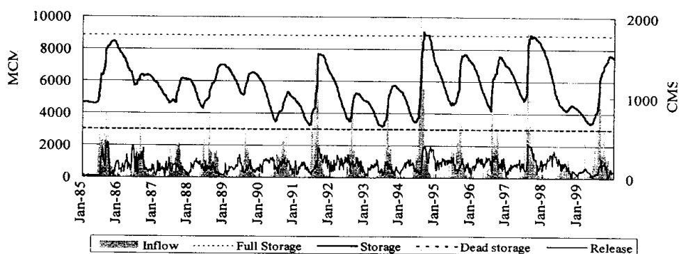
Fig. 2. Reservoir Operation Record (KHL)
