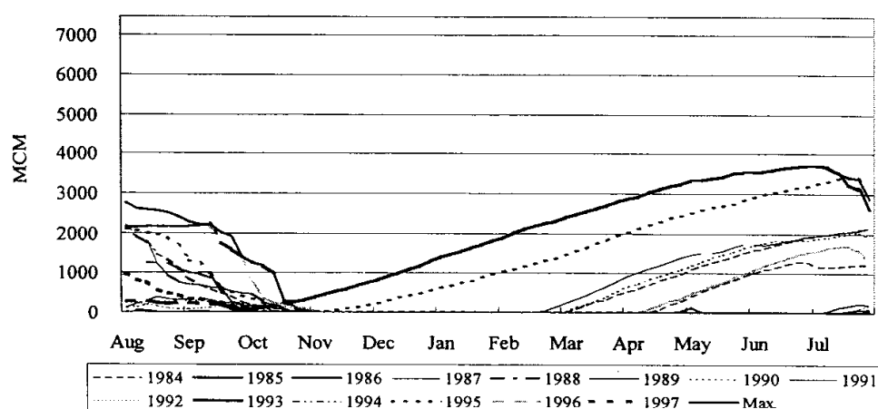
Fig. 7. Seasonal Vacancy Requirement (SRN)
