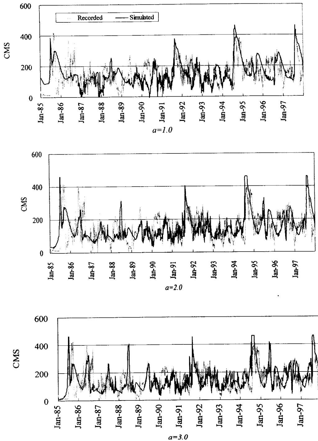
FIG. 14. SIMULATED RELEASE FROM KHL DAM AT DIFFERENT \alpha VALUES.
