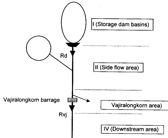
Fig. 4. Modeling of the Mae Klong River Basin
