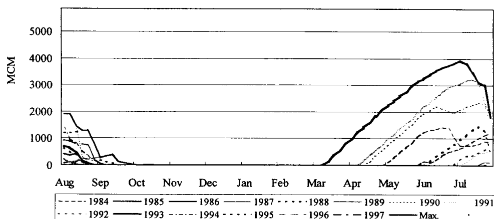
Fig. 8. Seasonal Vacancy Requirement (KHL)
