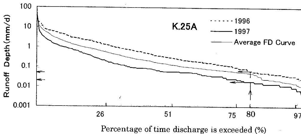
Figure 5. Flow duration curve for K.25A site.
