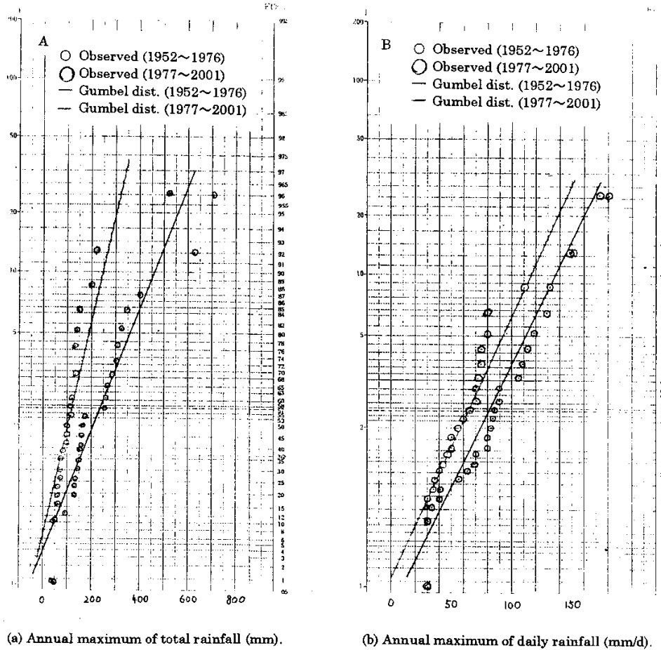
Figure 7. Plotting on Double exponential distribution paper.
