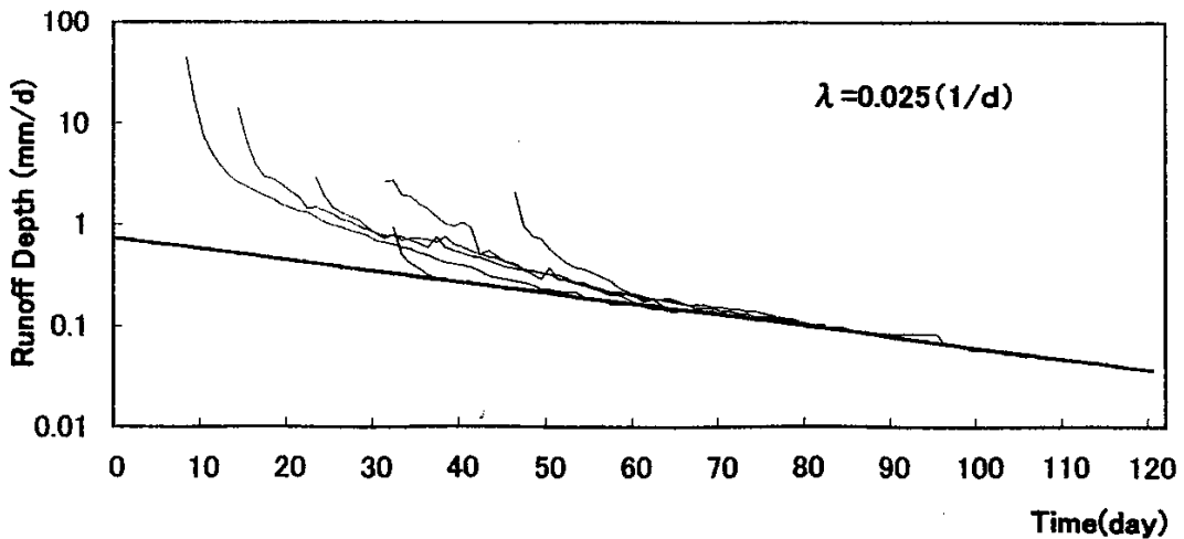
Figure 4. Master recession curve for the K.25A site.
