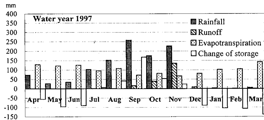
Figure 6. Monthly water balance.
