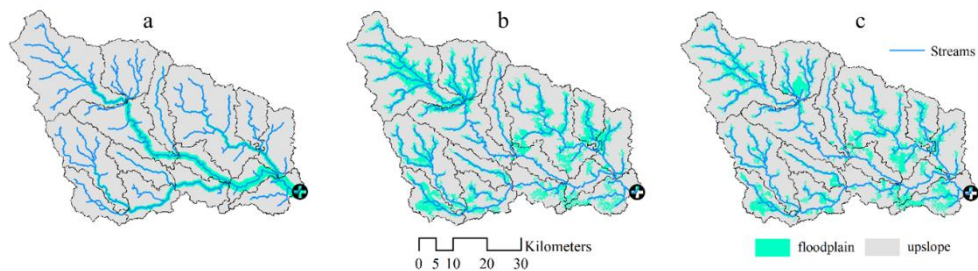
Fig. 3. Comparison of landscape units using three options available from the QSWAT+: (a) Buffer streams method, (b) DEM inversion method, and (c) Branch length method.
