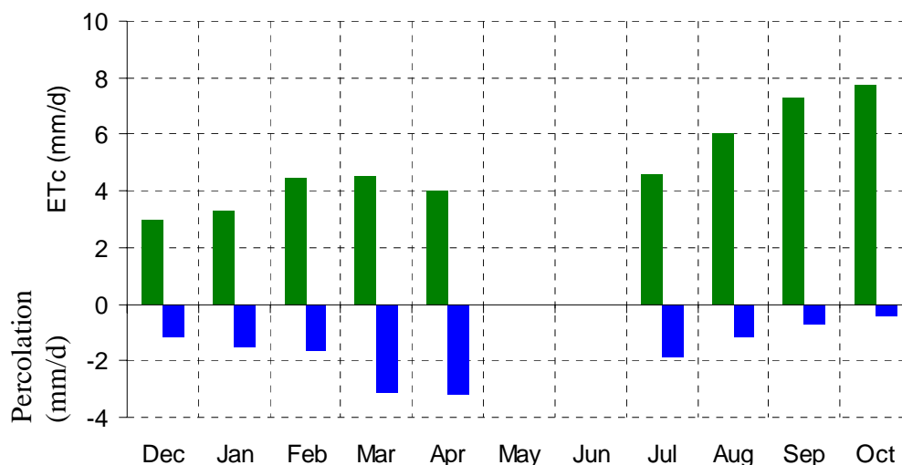
Figure 8: Evapotranspiration
