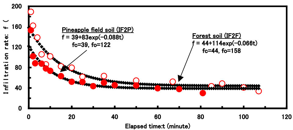
Fig. 11 Infiltration capacity curves of the forestland and the pineapple field at the IF2 site f: Horton equation, f_c : final rate, f_o : initial rate
