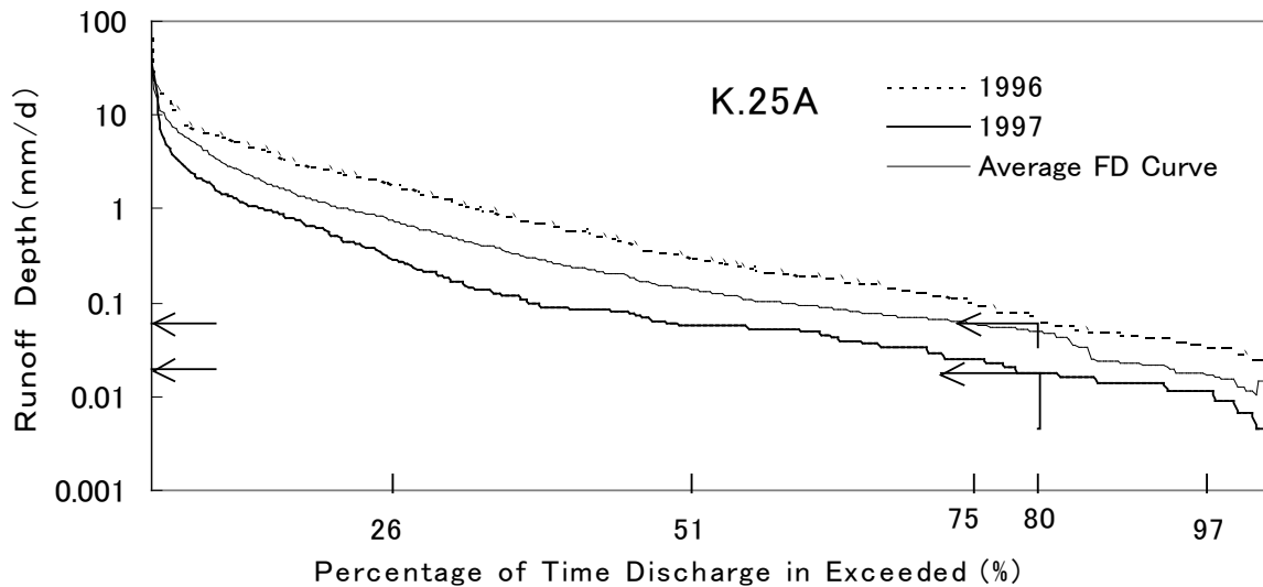
Figure 5. Flow duration curve for K.25A site.
