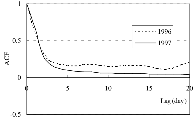
Figure 3. ACF of daily discharges
