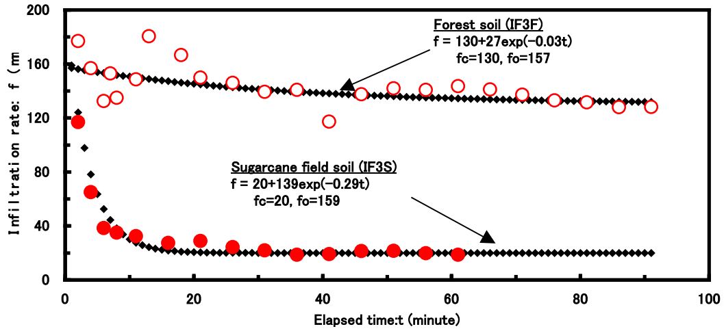
Fig. 12 Infiltration capacity curves of the forestland and the sugarcane field at the IF3 site f: Horton equation, f_c : final rate, f_o : initial rate
