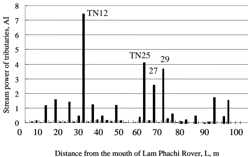
Figure 3. Calculated stream power of each tributary.
