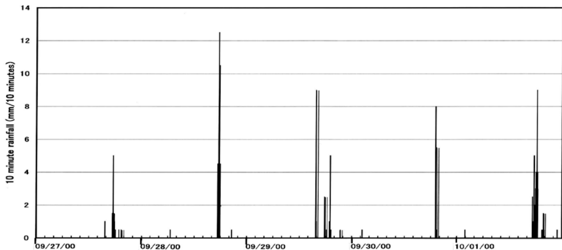
Fig. 15 10 minute rainfall from 27 September to 1 October 2000 at RGS
