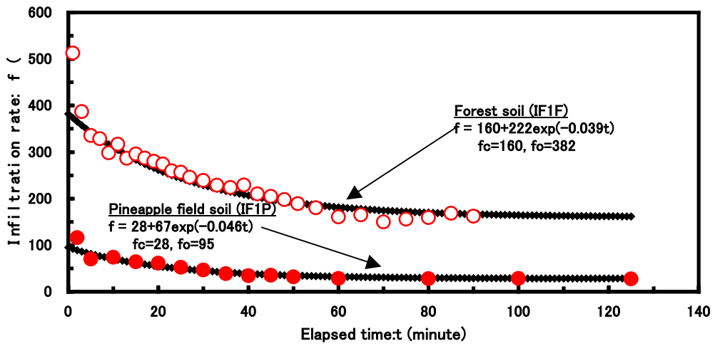
Fig. 10 Infiltration capacity curves of the forestland and the pineapple field at the IF1 site f: Horton equation, f_c : final rate, f_o : initial rate
