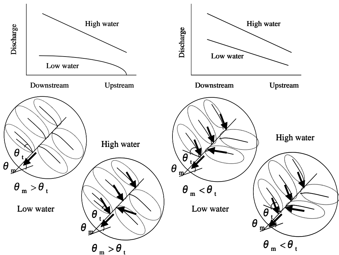
Figure 10. Idealized model of sediment and water discharge from tributary catchments under geomorphic control.
