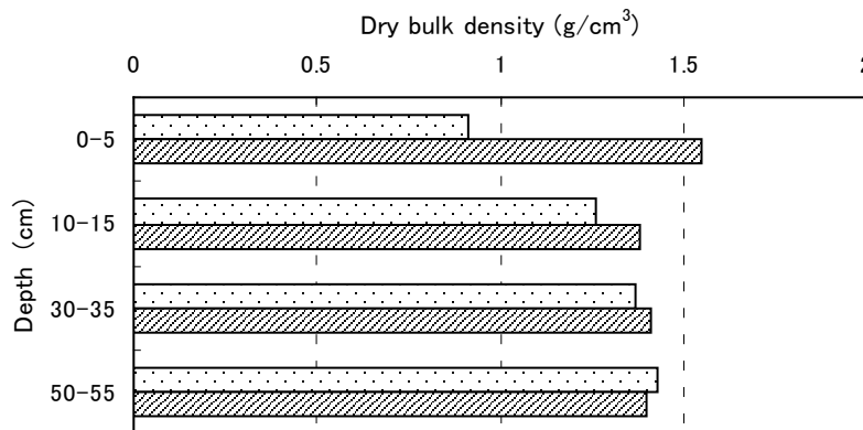
Fig. 5 Dry bulk density at each depth
